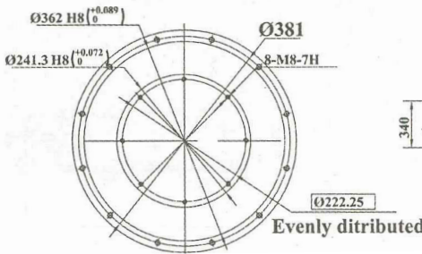
Connecting dimensions of flywheel and its housing
