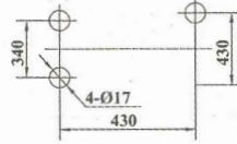
Flywheelhousing / Flywheel SAE4/7.5
