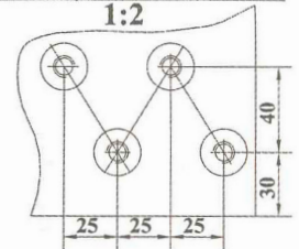
View B(cylinder block)
