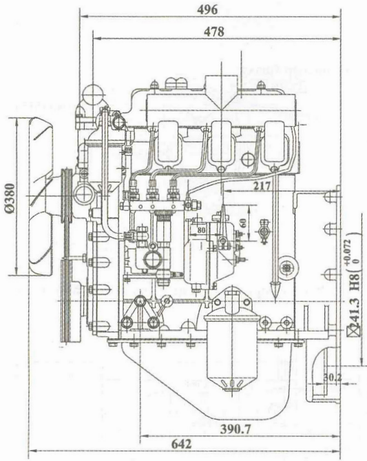
Connecting dimensions of flywheel and its housing
