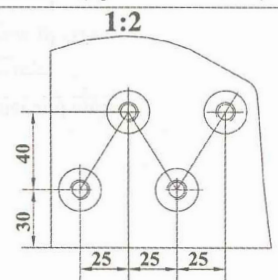
View B(cylinder block)
