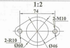
Dimensions of exhaust outlet
