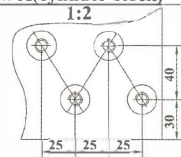
View B(cylinder block)
