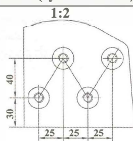
View B(cylinder block)
