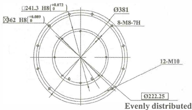
Connecting dimensions of flywheel and its housing
