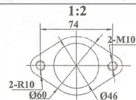
Dimensions of exhaust outlet
