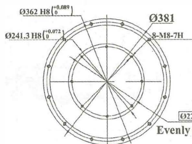
Connecting dimensions of flywheel and its housing
