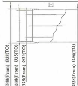
Dimensions of water inlet and outlet
