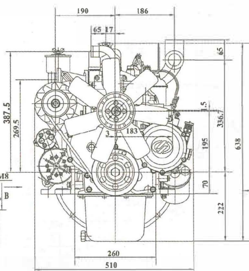
Dimensions of exhaust outlet centerline
